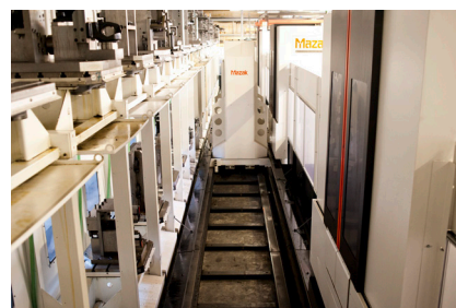
CELLULE FLEXIBLE
